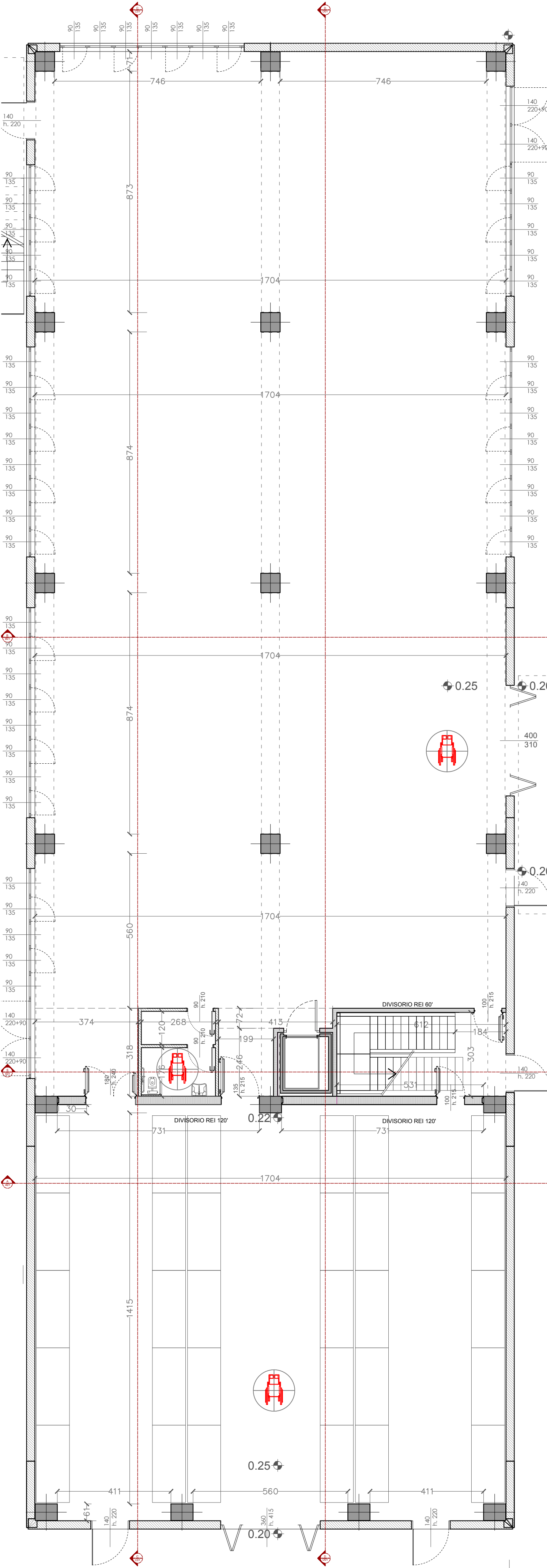
PIANO TERRA (+0.10)
